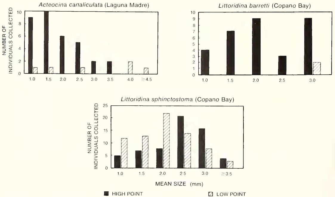
TEXT-FIG. 9. Comparison of the size-frequency distribution of species in the death assemblage just after an input pulse (the abundance high, see text-fig. 1) with the size-frequency distribution after taphonomic decay (the abundance low, see text-fig. 1).
